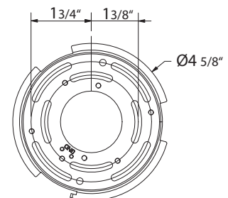
Mounting Backplate Dimensions
