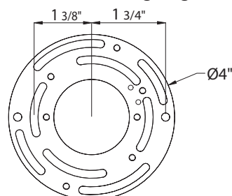
WS-72210 Mounting Ring
